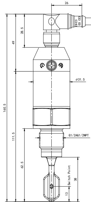
M12x1
